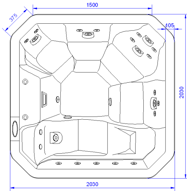
Drawing A1: Top view
